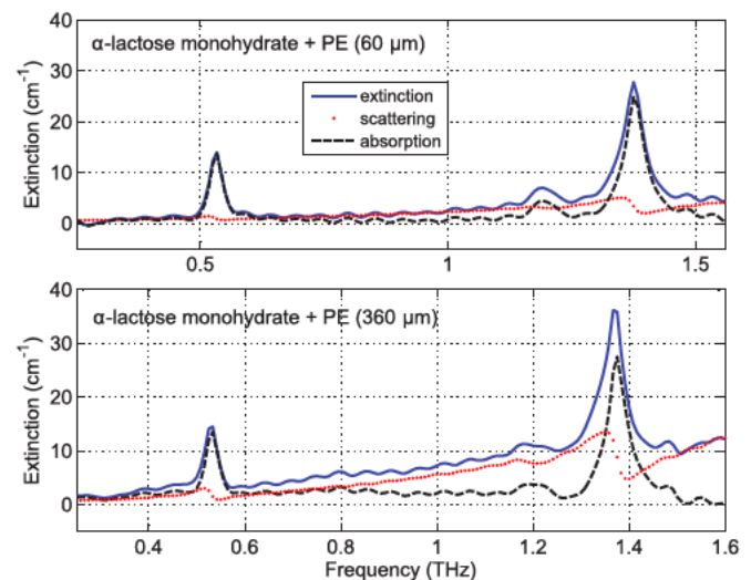
FIG. 2. Measured extinction spectrum (solid line), estimated scattering (dotted line), and scattering mitigated spectrum (dashed line) for alpha lactose monohydrate and PE samples.
