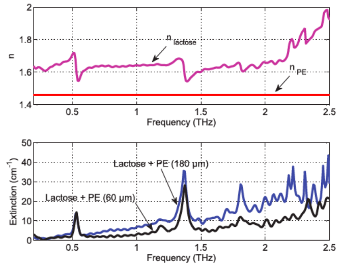
FIG. 1. Extinction coefficient and refractive index of the alpha lactose monohydrate and PE sample.
