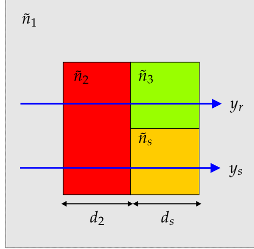
Figure 4.3. T-ray transmission notation for a single-thickness sample. This schematic shows the notation for modelling T-ray propagation through a sample slab, mounted on a substrate. The sample to be studied, with refractive index \tilde{n}_s , is attached to a substrate material with refractive index \tilde{n}_2 , and both are immersed in a medium of refractive index \tilde{n}_1 . The green area, \tilde{n}_3 , typically has a refractive index equal to \tilde{n}_1 or to \tilde{n}_2 , depending how the sample is prepared: if the sample is implanted into the substrate, \tilde{n}_3 = \tilde{n}_2 . If the sample is deposited onto the substrate, then \tilde{n}_3 = \tilde{n}_1 . In single-thickness measurements, the reference pulse y_r passes through the substrate then the green area. The spectral components of the waveforms are determined by FFT, \tilde{S}_s = \mathcal{FT}(y_s) and \tilde{S}_r = \mathcal{FT}(y_r) . Single-thickness samples are used for experiments in Chs. 6 and 7.
