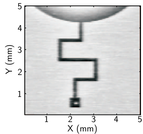
(b) Dynamic aperture near-field T-ray image
