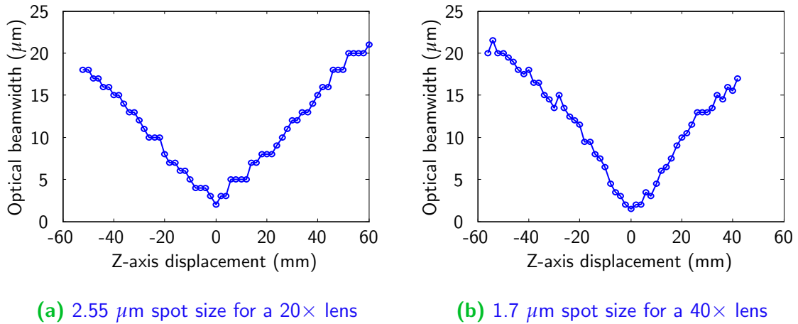
Figure 10.11. Measured focussed optical spot sizes. These plots show the measured optical spot size of focused optical beam using two objective lenses. The spot size was measured by scanning a sharp blade across the beam and estimating the distance over which the transmitted power dropped from 90% to 10% of the full, unobstructed optical power. These measurements indicate that the objective lenses used to generate sub- \lambda -sized T-rays were focussing as expected (Yuan et al., 2002).
