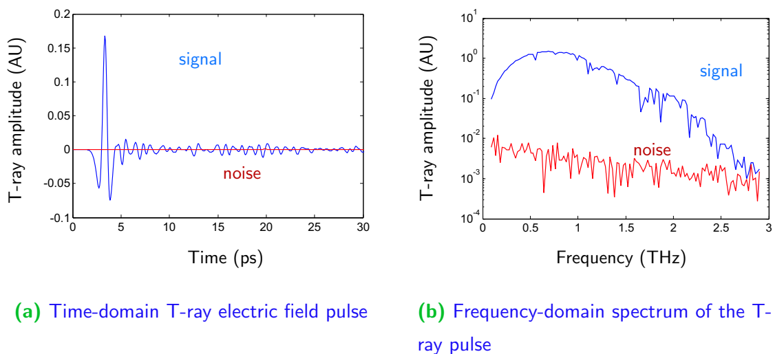
Figure 1.2. An example of a sampled T-ray waveform and its spectrum. Subfigure 1.2(a) shows an example of a T-ray pulse. The X axis shows the ps duration of the pulse. The Y axis shows the electric field amplitude of the broadband signal. Subfigure 1.2(b) shows the frequency-domain spectrum of pulse lying in the THz band. The pulse was measured experimentally on a typical T-ray spectrometer, described further in Ch. 3. The blue T-ray pulse is compared to the noise of the T-ray system in red, showing the high dynamic range of the T-ray spectrometer.
