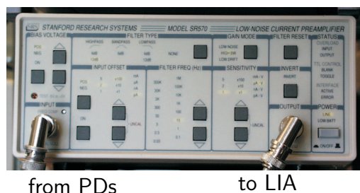
Figure B.10. Photograph of the low-noise current amplifier. Stanford Research Systems low-noise current preamplifier. The preamplifier took the current signal from the balanced photodetectors (PDs) and converted it to a voltage signal for the Lock-In Amplifier (LIA, see Sec. B.7.1). The main benefit of using the preamplifier was its adjustable gain-bandwidth product – the gain could be set sufficiently high to avoid any contributions from electronic noise without reducing the bandwidth below the modulation frequency (for example, the chopper frequency).
