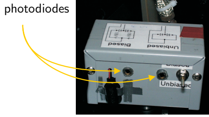
(a) Mounted balanced photodiodes and current difference circuit
