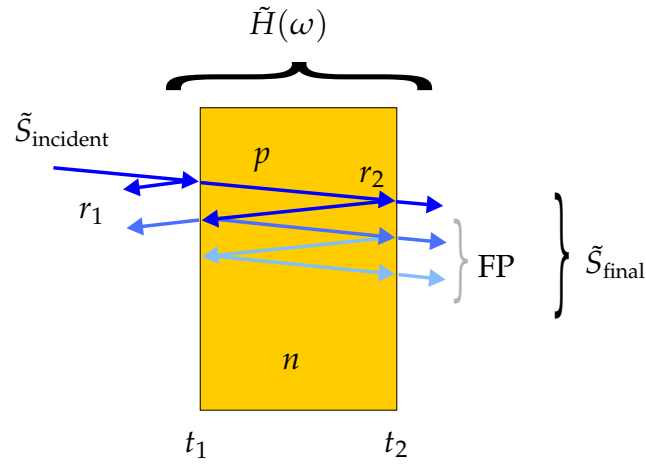
Figure 4.1. Multi-reflections and transmission through a dielectric slab. This Figure shows a dielectric slab of complex refractive index \tilde{n} , with an incident plane wave of electromagnetic radiation, represented by the single spectral component \tilde{S}_{\text{incident}} . Each spectral component represents a different frequency component of the plane wave (or equivalently, a different wavelength). The plane wave undergoes reflections r at the interfaces of the dielectric (first and second interfaces have coefficients r_1 and r_2 ), and propagates through p . Multi-reflections cause interference patterns in the final output wave, represented by the Fabry-Pérot factor, FP. The various coefficients are multiplied together to give a transfer function \tilde{H} for the dielectric slab.
