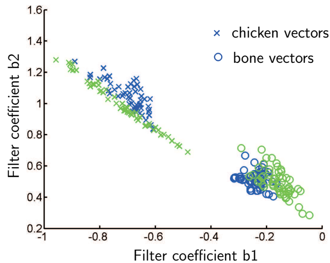
Figure 9.5. Classification results for measured bone and chicken spectra. This plot shows the effective classification of T-ray waveforms using coefficients b1 and b2 derived by fitting the data to one of two finite impulse response filters. The filters were developed with known training data. The fast algorithm clearly differentiates between bone and meat in this chart, depending only on the two coefficients (after Ferguson et al. (2001b)). The use of this classifier in imaging is shown in Fig. 9.6.
