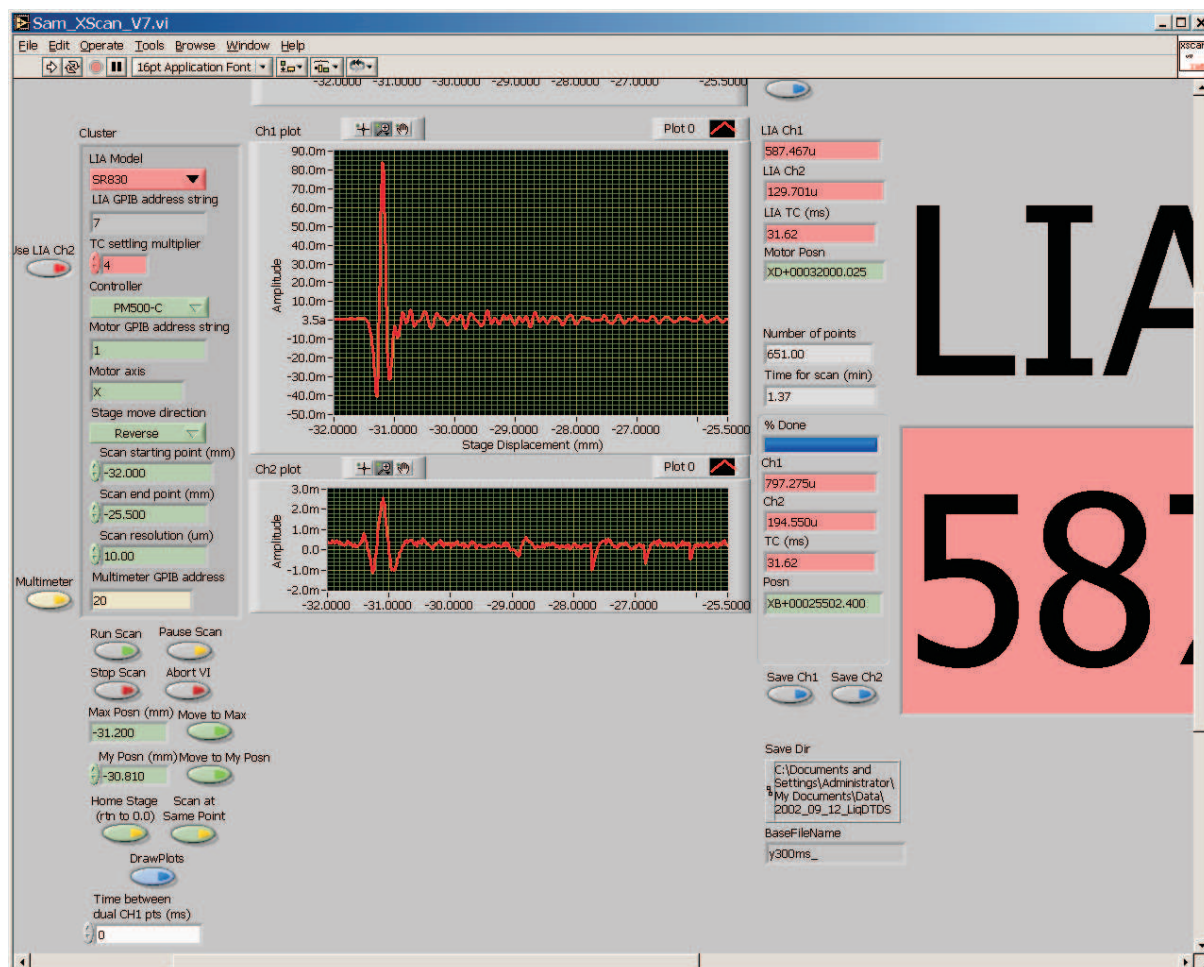
Figure B.5. Screen shot of control software for operating T-ray TDS experiments. This is a screen shot of the LABVIEW computer interface used to control the T-ray spectrometer used in this Thesis. The controls for the experiment are shown on the left and the readouts are on the right. In the centre is a large time-domain graph of a sampled T-ray waveform – the X-axis is a readout of the delay stage position and the Y-axis is channel one of the Lock-In Amplifier (LIAs). The smaller graph underneath shows channel two of the LIA, which should be much smaller than channel one if channel one is in phase with the optical modulator (chopper). The large display half-visible on the right-hand side was used for reading the LIA output from across the room when aligning certain optics.
