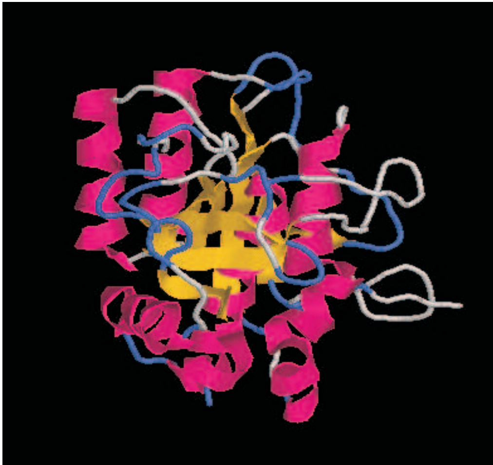
Figure C.1. Diagram of Subtilisin Carlsberg (SC) structure. This diagram outlines the structure of SC. The common formations of alpha helices (red) and beta sheets (yellow) are visible. This diagram was viewed using RASMOL (URL: http://www.rasmol.org ) from data in the Protein Data Bank (URL: http://www.rcsb.org ).
