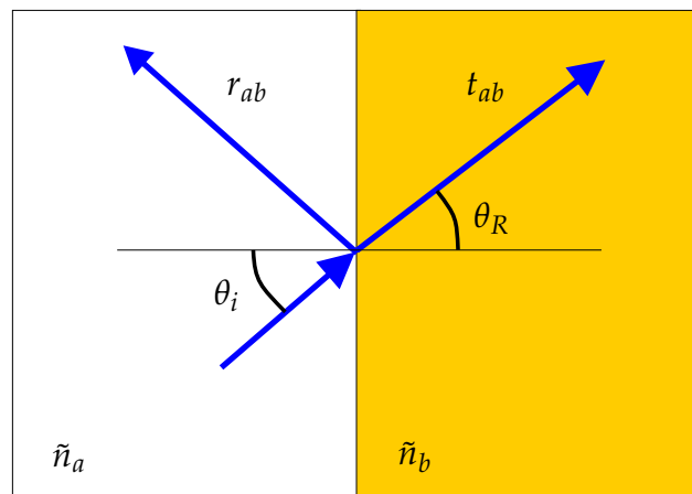
Figure 4.2. Fresnel coefficients. This diagram shows the notation for the reflection and transmission coefficients at a dielectric interface (Born and Wolf, 1997; Saleh and Teich, 1991).
