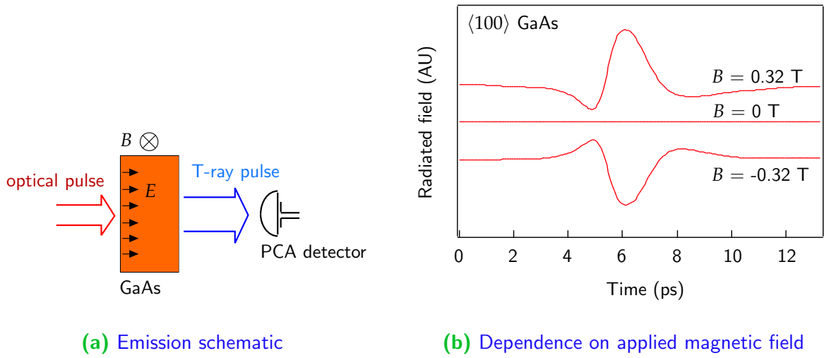
Figure 3.5. T-ray generation from an unbiased semiconductor in a magnetic field. The intrinsic bias field, E , is shown parallel to the page (that is, normal to front face of the semiconductor surface). The T-rays generated from an unbiased semiconductor are enhanced by the application of a DC magnetic field, B , shown normal to the page. The enhancement can be seen in Subfig. 3.5(b). This effect is discussed in Sec. 3.2.4. (After Zhang et al. (1993a).)
