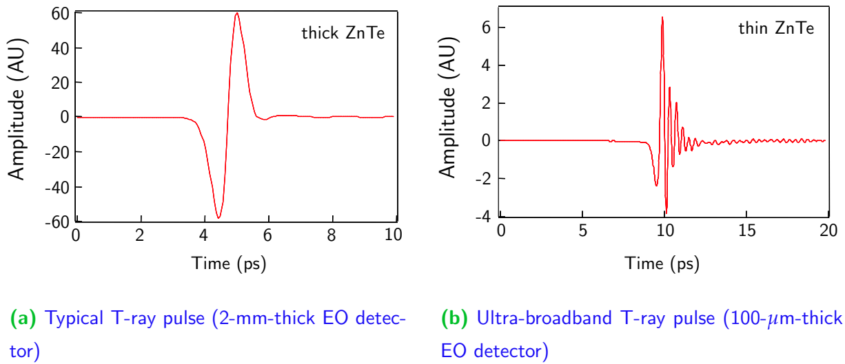
Figure 3.11. Measured broadband T-ray pulses. Crystal thickness determines signal sensitivity and bandwidth in EOS. The two Subfigures show a T-ray pulse sampled with two ZnTe detectors. Typically a 2-mm-thick ZnTe crystal provides a high signal, but a bandwidth limited to under 10 THz. ZnTe is a good EO sensor because of phase matching between the T-ray and optical pulses. Ultra-broadband phase matching is, however, not possible, so a thinner crystal detects higher frequencies. Using a 10- \mu m-thick crystal, frequencies up to 70 THz have been measured (Leitenstorfer et al., 1999). (After Han and Zhang (1998b).)
