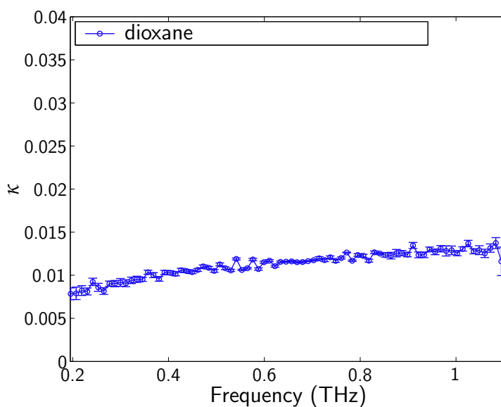
Figure 5.10. Measured T-ray absorption spectrum of dioxane. The absorption spectrum of dioxane was measured using dual-sample T-ray spectroscopy, described in Sec. 5.2. The bandwidth is limited to the region of maximum SNR. The error bars on the plot indicate the standard deviation over six separate samples.
