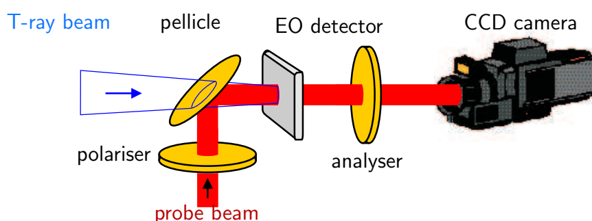
Figure 9.2. Diagram of CCD Electro-Optic Sampling. This schematic shows how Electro-Optic Sampling (EOS) can be implemented in 2D. As in normal EOS, described in Sec. 3.3.2, the T-ray beam is coincident with a polarised probe beam inside an EO crystal. Through the nonlinearity of the EO crystal, the electric field of the T-ray pulse rotates the polarisation of the probe beam. The extent of polarisation rotation is turned into an intensity modulation through an analyser (optical polariser oriented perpendicular to the first polariser). The intensity modulation of the probe beam is detected using a photodetector, or in the case of 2D EOS, an array of detectors. 2D EOS differs from point EOS in that both the probe beam and the T-ray beam are expanded onto the EO detector, and the transverse intensity modulation of the probe is detected by a CCD camera. The data is loaded directly to a computer for presenting a visual image. Three-dimensional data sets can be built up and analysed in XY slices, or with time on one axis. (After Wu et al. (1996c) and Wu et al. (1996a).)
