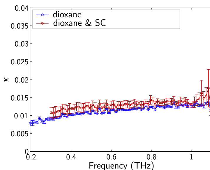
Figure 5.13. Measured T-ray absorption spectrum of dioxane & Subtilisin Carlsberg. The absorption spectrum of dioxane and 2 mg/mL of Subtilisin Carlsberg was measured using dual-sample T-ray spectroscopy, described in Sec. 5.2. The bandwidth is limited to the region of maximum SNR. The error bars on the plot indicate the standard deviation over six separate samples.
