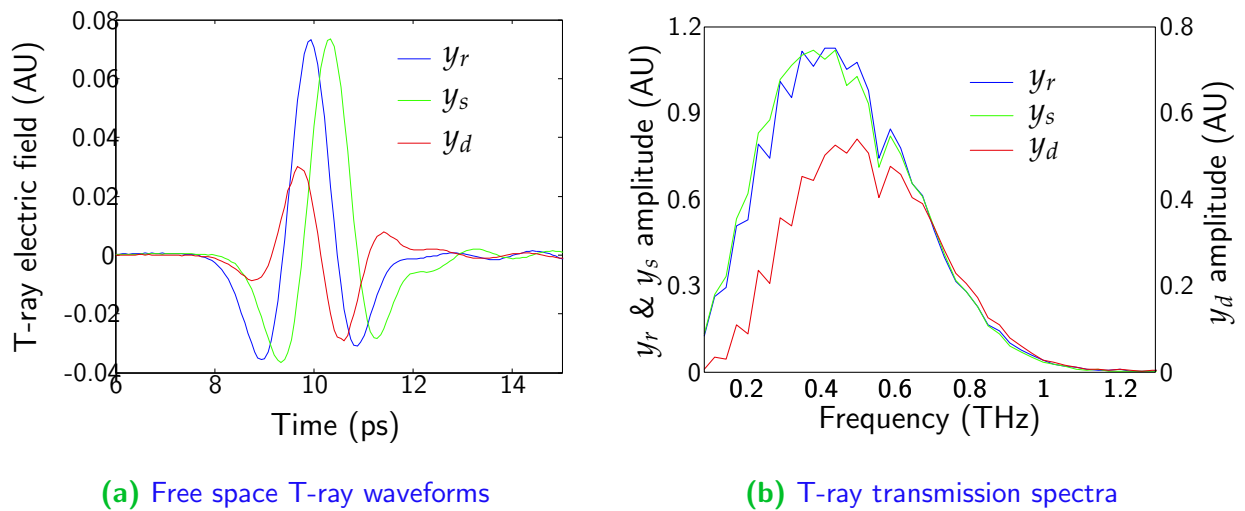
Figure 6.14. Measured DTDS waveforms and spectra. These two graphs compare the differential pulse to the reference and sample pulses in both the time and frequency domain. The reference pulse y_r has the largest amplitude. The sample pulse y_s has a reduced amplitude and phase shift, which is characteristic of the material being studied. The differential pulse is the difference y_d = y_r - y_s . The differential pulse also approximates the slope of y_r , as discussed at the start of Sec. 6.2.1. These measurements were taken with a LIA time constant of 100 ms, at room temperature. The bandwidth of the reference pulse is typical for a T-ray system, driven as it is by T-ray generation from a GaAs surface using 100-fs optical pulses. The absorption lines in all three spectra, at 0.56, 0.75 and 1.1 THz, were caused by water vapour in the air (van Exter et al., 1989b).
