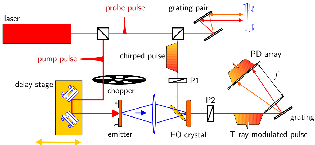
Figure 3.12. Single-shot detection. This schematic shows the chirped pulse single-shot T-ray pulse detection technique. The single-shot spectrometer is similar to a typical T-ray detection system, using OR and EOS, except the probe pulse is stretched to a ps duration with a grating pair. The polarisers 'P1' and 'P2' are used for crossed polarisation detection (see Sec. 3.3.2). When the T-ray and probe pulses propagate collinearly through the EO detector, they both have approximately the same duration, thus different wavelengths in the spread probe pulse experience different levels of intensity modulation. As the pulse is chirped, these different levels are separated with a spectral grating, and detected with a linear photodiode (PD) array. A lens with focal length f focuses the pulse onto the array. Apart from a background measurement of the unmodulated chirped pulse required to extract the T-ray waveform, the technique can measure the entire T-ray waveform in a single shot. The T-ray wavefront is focused from emitter to detector in this scheme with a polyethylene lens, which has a very low dielectric constant for T-rays. The purpose of this particular configuration is to study the propagating wave shape; for material measurements, a sample can be placed between two polyethylene lenses ( 2f spacing) in the T-ray beam path. For single-shot imaging, discussed in Sec. 9.4, the T-ray beam is spatially expanded in 1D and the PD array is replaced with a CCD. (After Jiang and Zhang (1998a).)
