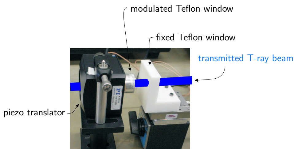
Figure 11.8. Piezoelectric sample modulator concept. This photograph shows how a piezoelectric positioner might be used to implement liquid DTDS with sufficient accuracy to improve the noise performance by over two orders of magnitude (from Fig. 8.17).
