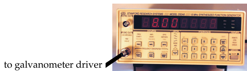
Figure 6.9. Photograph of a function generator used for double-modulated DTDS experiments. A Stanford Research Systems DS340 function generator was set to generate a sinusoidal 8.0 V peak-peak amplitude, which drove the DTDS galvanometer at 1 cm peak-to-peak.
