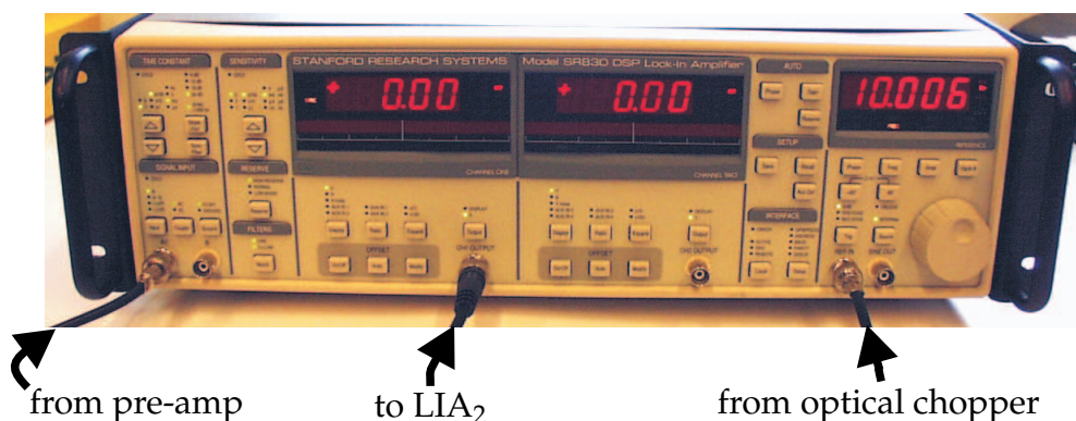
Figure 6.7. Lock-In Amplifier (LIA) photograph. This picture shows the front panel of a Stanford Research Systems LIA used in the double-modulation detection scheme. The signal from balanced photodiodes is amplified by a current amplifier, then input to the LIA for demodulation and low-pass filtering. The settings on the LIA are set manually using the front panel or using General Purpose Interface Bus (GPIB) commands from the computer. A more detailed description of this LIA, the SR830 DSP, is given in Sec. B.7.
