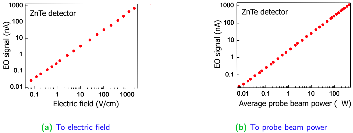
Figure 3.10. Measured linearity of ZnTe EOS. These results demonstrate the linearity of ZnTe as a T-ray sensor, to both the probe beam power and the T-ray electric field. The linearity is ( <2\% ) for over more than 5 orders of magnitude. (After Wu et al. (1996c).)
