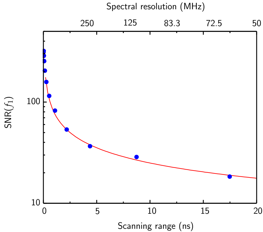
Figure A.5. Measured SNR of T-ray TDS at one frequency ( f_1 ) versus scan duration. This graph shows the variation of the SNR of T-ray TDS at one frequency as a function of the temporal scanning range \mathcal{T} . The frequency chosen for these measurements was the frequency that had the highest amplitude. The solid dots are experimental data and the curve is fitted the calculated results from Eq. (A.8), thus confirming its accuracy. The experimental conditions are described in Sec. A.3. The spectral resolution \Delta f is also shown in this graph, and is inversely proportional to the scanning range \mathcal{T} .
