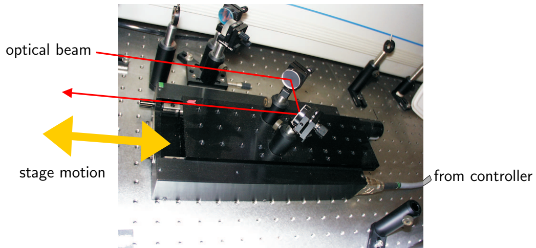
Figure 3.7. Pump-probe delay stage. The delay stage pictured here is the essential element in pump-probe experiments, of which T-ray spectroscopy is one example. The stage is used to sweep the ultrafast probe pulses over the temporal profile of the free-space T-ray pulse, thereby sampling the entire T-ray waveform. The stage motion is coordinated with the detection electronics via a computer and General Purpose Interface Bus (GPIB)) interface.
