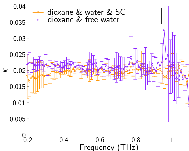
Figure 5.16. Measured absorption of dioxane & free water. This Figure compares the measured absorption spectra of mixtures of dioxane and free water to dioxane and water and SC. The data were measured using the T-ray spectrometer as described in Sec. 5.2. The bandwidth is limited to the region of maximum SNR. The error bars on the plots indicate the standard deviation over six separate samples.
