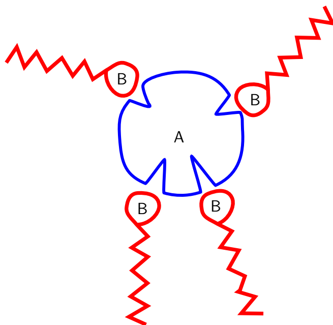
Figure 7.2. Sketch of Biotin and Avidin molecules. This sketch shows sketches of the molecules Biotin (marked 'B') and Avidin (marked 'A'). The essential characteristics of Biotin are the polar head and long non-polar tail. Avidin, a protein, has four binding sites for Biotin. Biotin-Avidin binding is sketched in Fig. 7.11. The molecules are not to scale.
