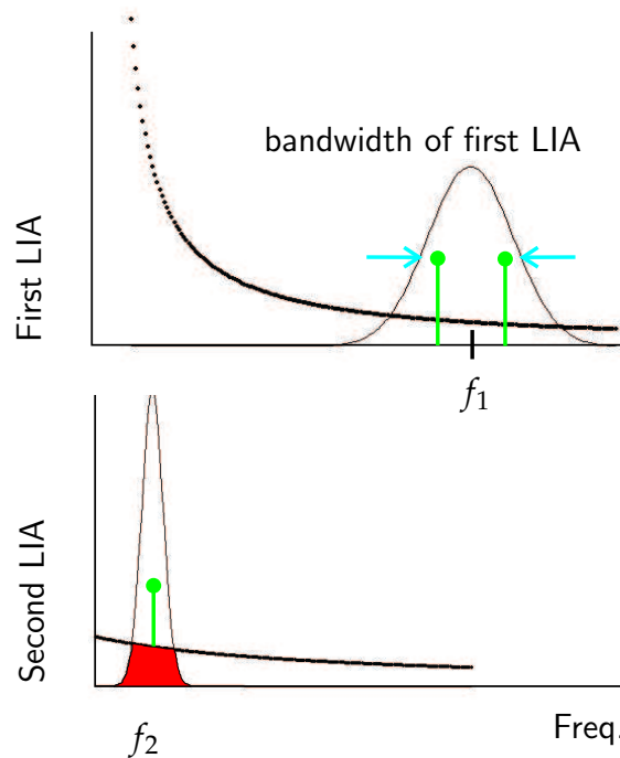
Figure 6.6. Explanation of double-modulation. These graphs outline the operation of double-modulation. In double-modulation, the signals at the input to the first LIA are found at the sum and difference of the modulation frequencies, f_1 + f_2 and f_1 - f_2 . The first LIA acts as a frequency mixer and demodulates the f_1 frequency, so that at the input of the second LIA, the signal is modulated at f_2 . One important point is that the bandwidth of the first LIA has to be set sufficiently wide to allow the signal to pass through at a frequency \pm f_2 from the centre frequency (Hemenway et al., 1987; Zhang et al., 1999).
