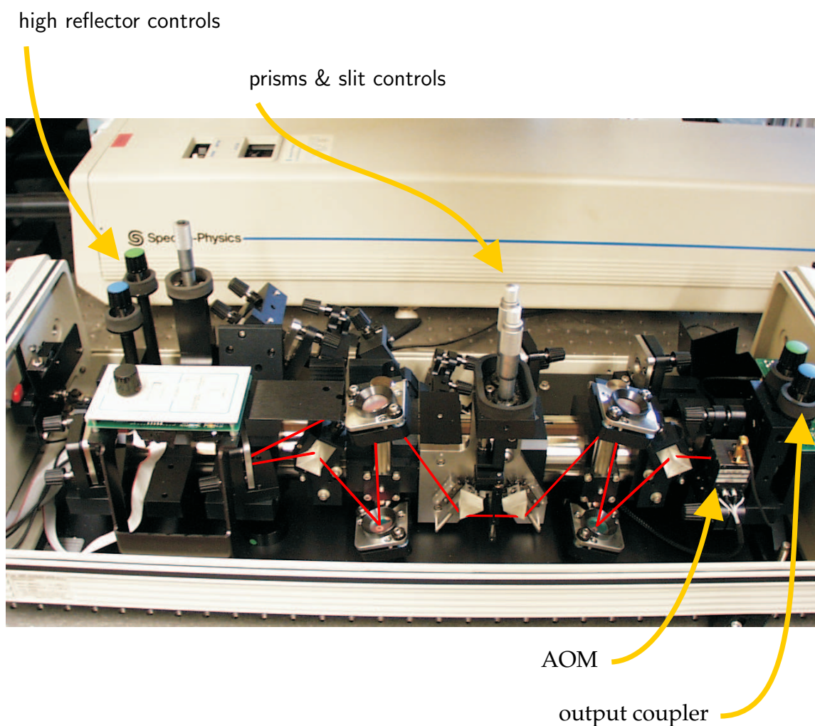
Figure B.2. Photograph of an ultrafast laser – open. This photograph shows the interior of the femtosecond laser used in most experiments in this Thesis (model: Tsunami, manufacturer: Spectra Physics, Mountain View, CA, USA; URL: http://www.spectraphysics.com ). Visible in this diagram is the Acousto-Optic Modulator (AOM unit, used to sustain mode-locking (pulsed operation) over long periods of time. The path of the laser beam is marked in red, refracting through the four dispersion-control prisms and into the AOM and output coupler (from left to right).
