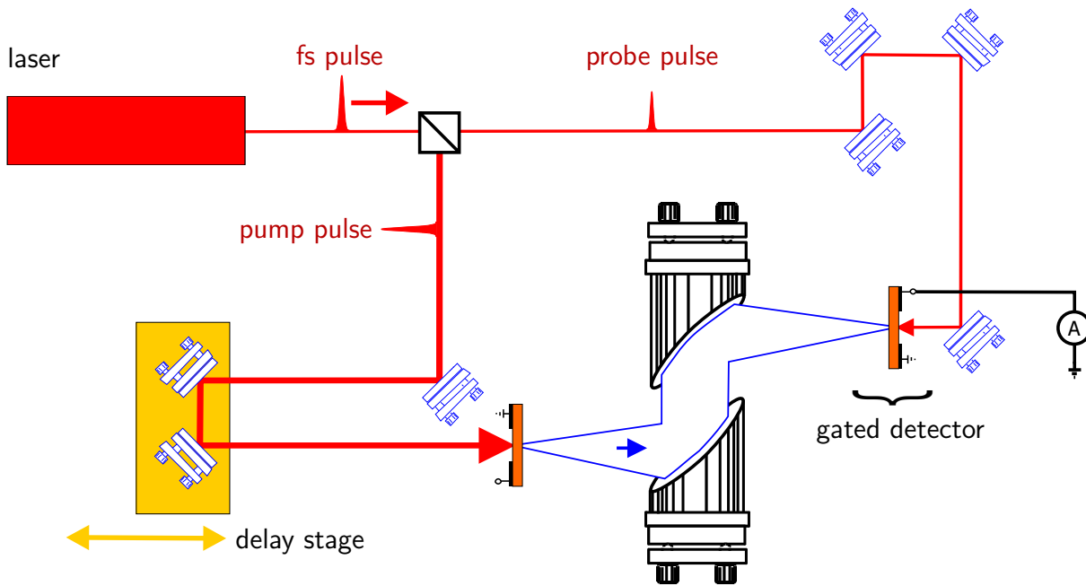
Figure 3.6. Schematic functional diagram of gated detection. This T-ray generation and detection schematic is an example of a pump–probe experiment. The pump beam initiates a T-ray pulse, which is detected by a gated detector. The gated detector is activated by the probe pulse. The time delay is varied with a delay stage. Thus the time evolution of the pulse can be sequentially sampled. The extra distance in the probe pulse path is required so that the optical path lengths of the pump and probe pulses are identical – the probe beam must gate the detector at the same time as the T-ray pulse arrives at the detector. In this example, PCAs are depicted as the T-ray emitter and detector. (Note that this bare bones schematic only shows the system components that are relevant to gated detection. Typical auxiliary elements in a T-ray spectrometer, such as the optical chopper, are not essential to gated detection.)
