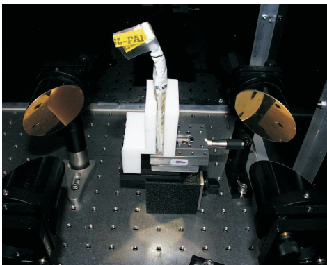
(a) Variable-thickness sample holder
