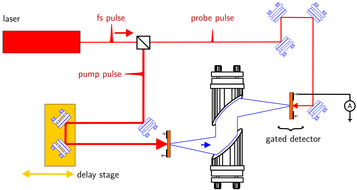
Figure B.11. Gated detection schematic. This T-ray generation and detection schematic is an example of a pump-probe experiment (from Fig. 3.6.)
