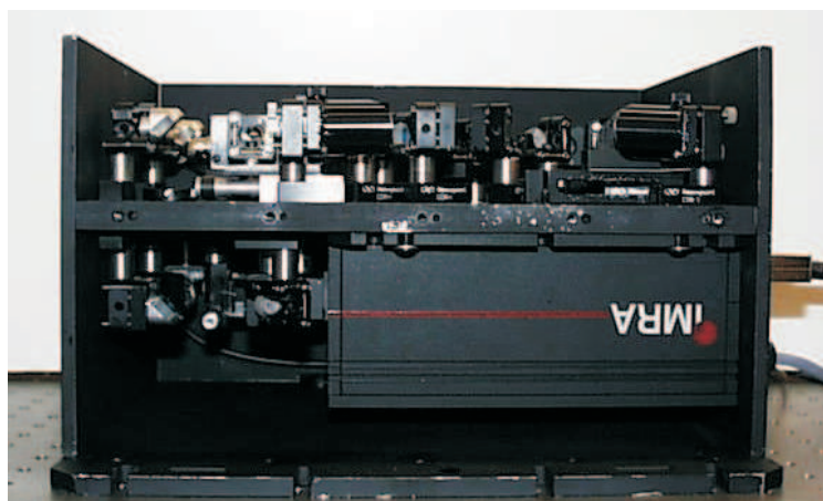
Figure 11.6. Compact T-ray spectrometer. This photograph shows a compact T-ray system, based on a fibre laser (manufacturer: IMRA America Inc., Ann Arbor, Michigan, USA; URL: http://www.imra.com ), sitting on a table with one-inch spaced holes (after (Li et al., 1999b)).
