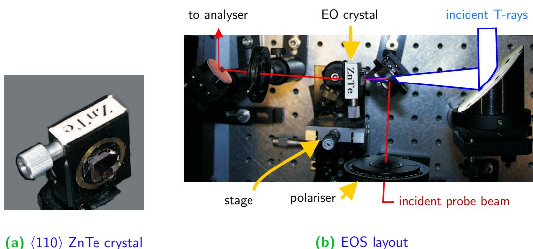
Figure 5.5. Electro-Optic Sampling. These pictures show the experimental layout of T-ray Electro-Optic Sampling (EOS) used in the experiments in this Thesis. EOS is the most sensitive, broadband technique of gated T-ray detection. The T-ray beam is focussed into the detection crystal using a gold-coated parabolic mirror. A pellicle directs the optical probe beam to travel collinearly with the T-rays through the crystal. The T-ray electric field rotates the polarisation of the probe beam. ZnTe is commonly used for EOS since the T-ray and optical pulses traverse it with similar velocities. The crystal is mounted in a rotating stage as the orientation of the EO crystal is critical to the sensitivity of the detection.
