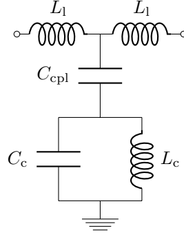
Figure 5. Equivalent circuit model of a microstrip line loaded with a pair of complementary split ring resonators (CSRRs).
