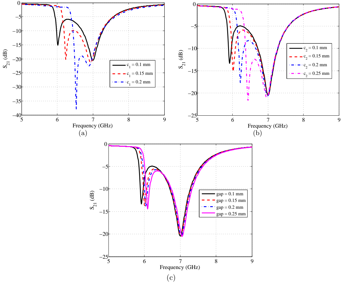
Figure 7. Simulation results for the S_{21} of a microstrip line loaded with a CSRR-DGS. The results show that any change in c_1 , c_2 and gap size only changes the resonance frequency of the CSRR and does not have a significant effect on the DGS resonance frequency.
