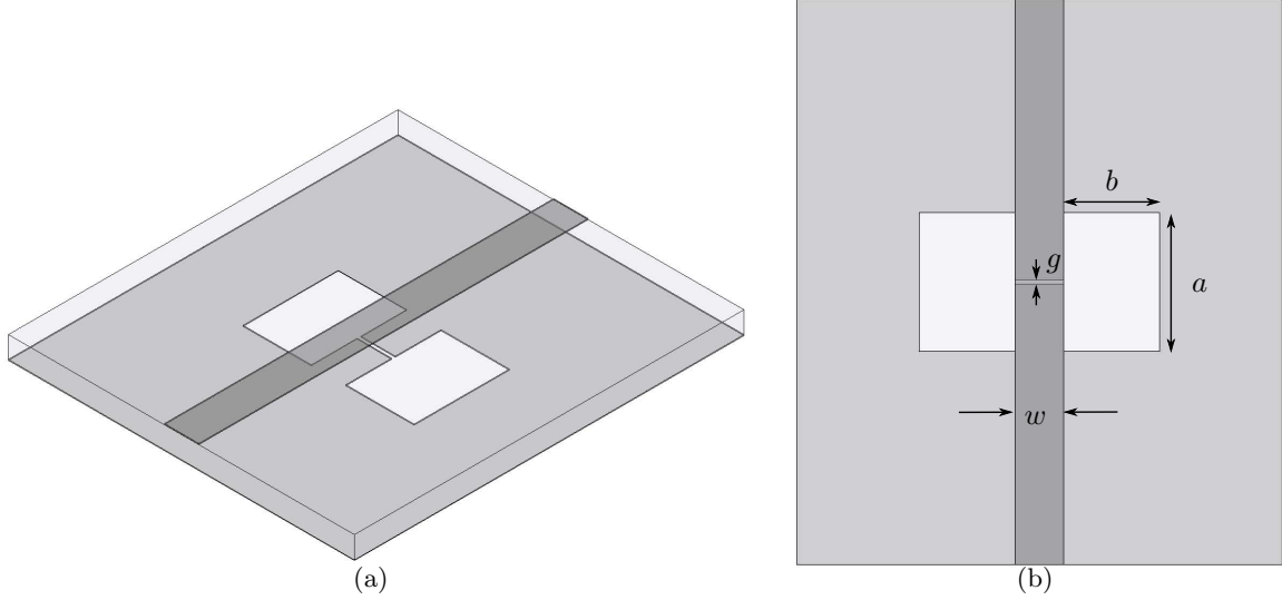
Figure 1. A 3D view (a) and a top view (b) of a microstrip line loaded with a dumbbell shape defected ground structure.
