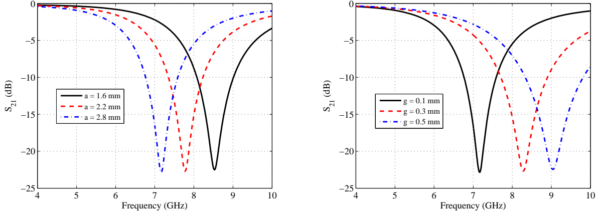
Figure 2. Variation of the resonance frequency in terms of (a) the rectangular defect width a , with g = 0.1 mm and (b) the slot width g , with a = 2.8 mm. The substrate thickness is 1.65 mm with a relative permittivity of 10 for all cases.
