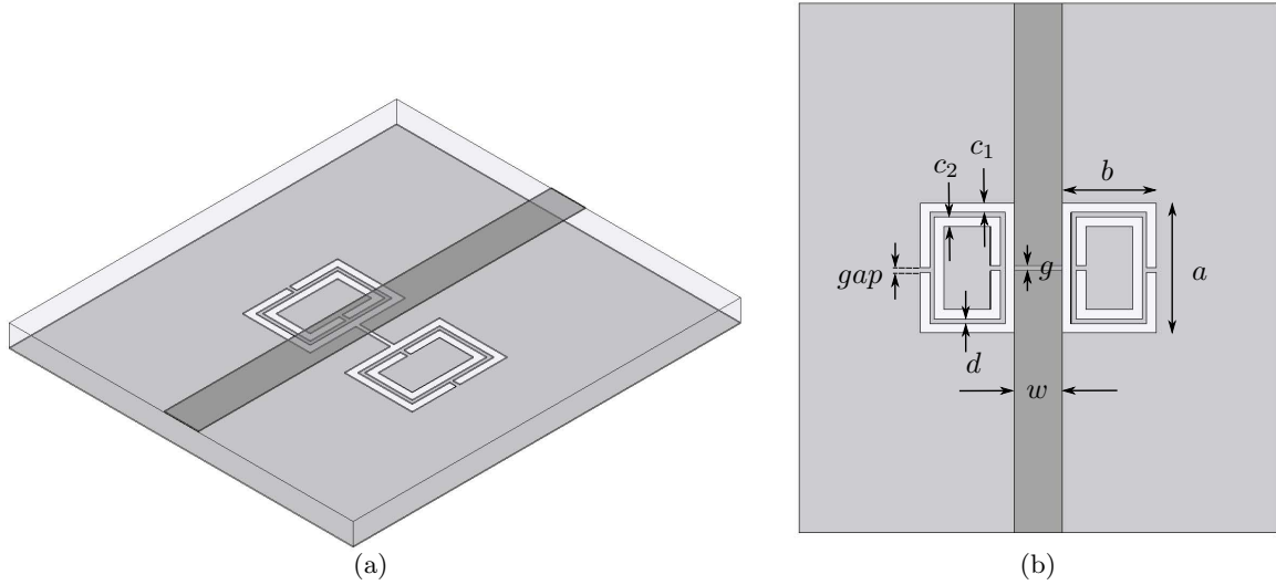
Figure 6. Three dimensional and top view of a microstrip line loaded with a CSRR-DGS. The structure can be either considered as a pair of complementary split ring resonators connected to each other through a slot or two CSRRs embedded inside the rectangular defect of a DGS.
