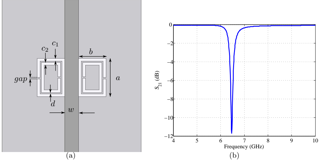
Figure 4. Microstrip line loaded with a pair of complementary split ring resonators (CSRRs), (a) the top view and (b) the simulated transmission coefficient of the structure in dB.
