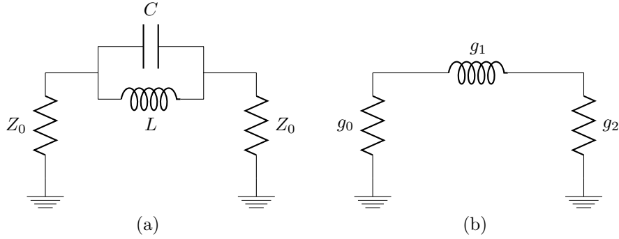
Figure 3. (a) Equivalent circuit of the microstrip line with dumbbell shape defected ground, and (b) one-pole Butterworth lowpass filter prototype.
