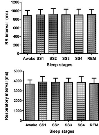
Figure 1. Average R-R and respiratory interval for different sleep stages.
