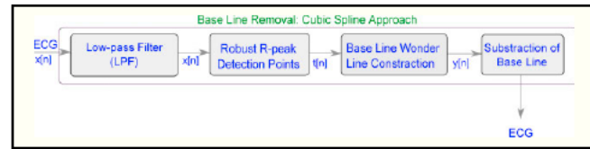
Figure 2. Baseline wander removal steps
