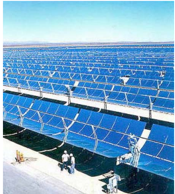
Fig. 3. The Solar Energy Generating Systems (SEGS) solar trough farm at Kramer Junction, California. The concept is that the reflective troughs focus sunlight on a pipe containing oil in a closed-cycle, which heats water to create steam to turbines. In total there are nine SEGS farms, with two at Daggett, five at Kramer Junction, and two at Harper Lake; all in California's Mojave Desert. The total area occupied is 2.4 sq km, generating 354 MW of power. These figures scale up to a footprint of 320 km by 320 km, if we were to supply 15 TW with this method. The nine plants have gradually been installed from 1984 to 1990, demonstrating over 20 years of performance without malfunction. Source: Power Corp.
