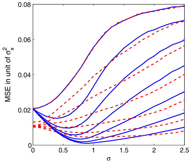
Fig. 3. The MSE distortion of weighting before summation versus the ratio of \sigma for uniform signal and noise distributions (from top to bottom, N = 1, 3, 7, 15, 31, 63 , and 127 ). The red dashed lines show the MSE distortion for the unique threshold setting, and the blue solid lines correspond to the MSE distortion of the identical threshold setting. The optimal weights for each comparator are solved using Eq. (10) with K = 10^6 data samples. (For interpretation of the references to color in this figure legend, the reader is referred to the web version of this article.)
