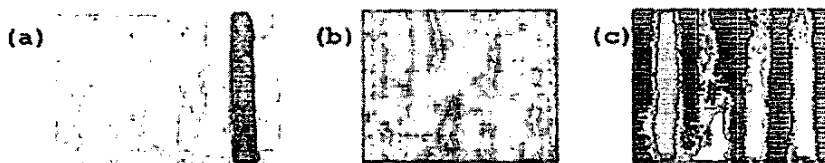
JMC2 Fig. 1. The powders used to demonstrate THz imaging. Figure (a) shows the piece of paper containing samples of salt, baking soda, flour and seasoning (from left to right). Figure (b) shows the THz image at a frequency of 0.3 THz. Figure (c) shows the results of classifying the THz data as described in the text. The image consists of five shades of gray. From darkest to lightest they correspond to paper, salt, baking soda, flour and seasoning.
