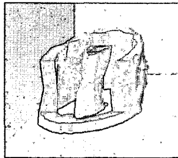
JMC3 Fig. 3. Reconstructed 3D image of the vial and plastic tube. Part of the data has been cut away to allow the interior of the vial to be viewed.
