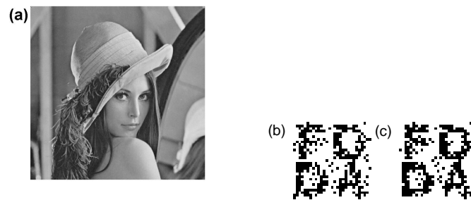
Figure 7. (a) JPEG compressed version of the marked image 'Lena' with 75% quality and 0% smoothing. The recovered binary image via (b) the isolated bistable detector, and (c) the array of bistable detectors with optimal noise intensity D_\eta/\Delta t = 100 . Here, \tau_a = T_b/150 , X_b = 3.75A and the array size N = 60 .
