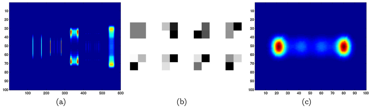
Fig. 16. Illustration of three-dimensional mirror symmetry analysis of a spherical object. (a) Non-negative tensor decomposition. (b) Sparse texture extraction. (c) Synthesis of the extracted texture.
