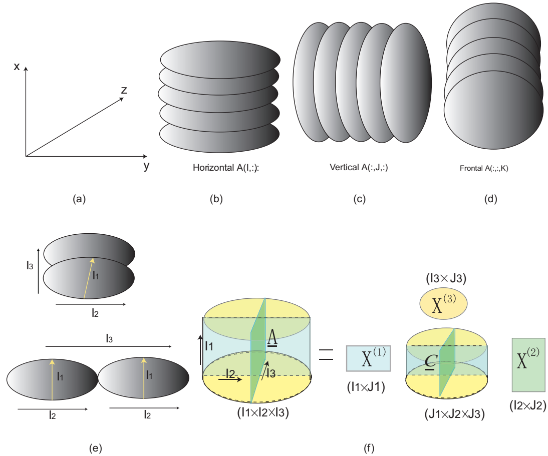
Fig. 15. (a) Illustration of the directions regarding the x-, y-, and z-axis. (b), (c), and (d). Illustration of three direction slices of a third order tensor: horizontal, vertical, and frontal, respectively, which are perpendicular to the x-, y-, and z-axis, respectively. (e) Illustration of the way to flatten the third order tensors along frontal slices. The colon (:) used in the figure indicates all the column elements at a given direction are involved to form an image matrix. (f) Illustration of a third-order decomposition.
