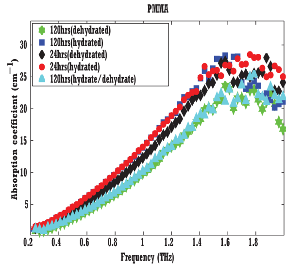
Fig. 2. (Color online) Absorption spectra of PMMA. This figure illustrates the absorption coefficient of PMMA at different hydration levels. It can be observed that there is a distinct difference between the hydrated and the dehydrated state. Also, it is noted that the hydration state of PMMA saturates after 24 h. The hygroscopicity measurement indicates that the PMMA absorbs 0.75% of water after 24 h and 1.8% after 120 h of hydration. The increase in absorption after the hydration for 24 h and 120 h is due to its methyl ( \text{CH}_3 ) polar group, which binds strongly to water molecules.
