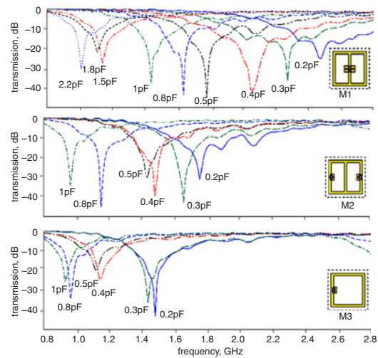
Fig. 2 Transmission magnitude of three resonators with different loaded capacitors
