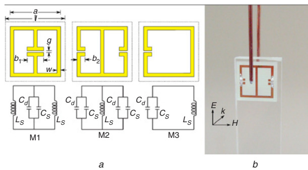
Fig. 1 Schematics of three metamaterial elements and their equivalent circuits (distributed capacitance and inductance denoted by C_s and L_s , respectively, and lumped capacitance denoted by C_d ), and photo of experimental setup showing resonator inserted between two monopole antennas
