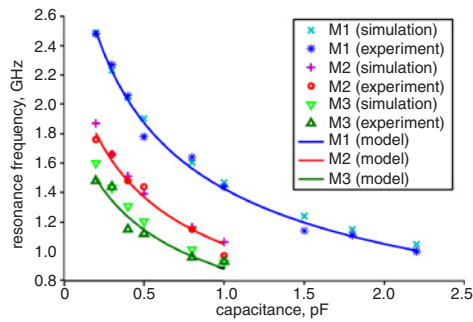
Fig. 3 Measured and simulated resonance frequencies against loaded capacitance
