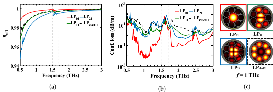
Figure 5. Simulated (a) \eta_{\text{eff}} ; (b) confinement loss; and (c) spatial electric field E distribution of AR fiber for the \text{LP}_{01} , \text{LP}_{11} , \text{LP}_{21} , and \text{LP}_{\text{clad01}} mode. The fiber has 140 metal-wire inclusions, a uniform wire diameter d = 90 \mu\text{m} and fixed dielectric thickness between the internal side of the metal wire and the inner dielectric cladding layer p = 289 \mu\text{m} .
