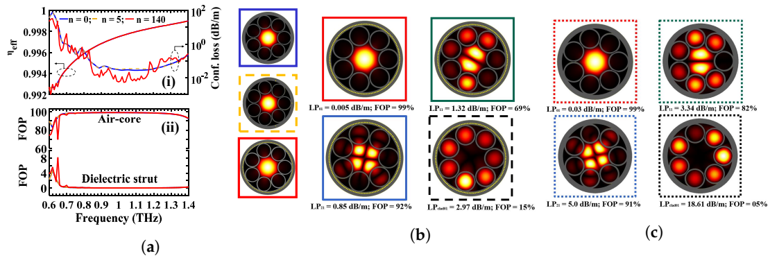
Figure 4. (a) Simulated (i) refractive index ( \eta_{eff} ) in left axis and confinement loss of LP_{01} -like fundamental mode in right axis; fraction of power in (ii) air core ( FOP_{core} ) at top and Zeonex strut ( FOP_{strut} ) at bottom. The simulations are performed by varying the metal wire numbers, n = 0, 5 , and 140. The fiber has a uniform wire diameter d = 90 \mu m and fixed dielectric thickness between the internal side of the metal wire and the inner dielectric cladding layer p = 289 \mu m . Spatial electric field E distribution for the modes in the (b) AR fibers with metal-wire inclusions and (c) AR fibers without metal-wire inclusions: LP_{01} , LP_{11} , LP_{21} , and LP_{clad01} (from left to right) at 1.03 THz.
