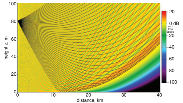
Fig. 5 Predicted field relative to free-space, and ray tracing, for p=0 Sub-refraction +400 M-units/km: M(0)=300 , M(80)=332 Transmitter: 10 GHz at 80 m. G_M=0.12 M-units/m and z_0=0.05 m
