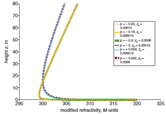
Fig. 1 Modelling two different ducts, each with three different values of z_0 . Refractivity profiles for M(0) = 320 , M(15) = 300 and G_M = 0.12 M -units/m, the two duct profiles being generated firstly with the usual z_0 value for evaporation ducts of 0.00015 m, and then super-imposed profiles with smaller and larger z_0 values, produced by adjusting the value of p in (4)
