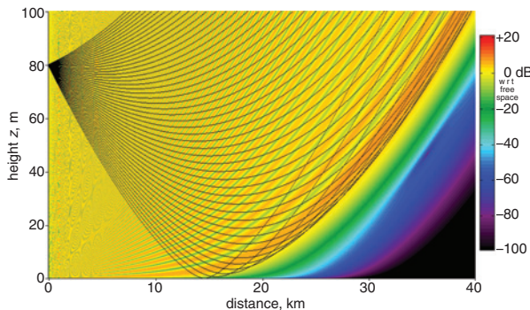
Fig. 4 Predicted field relative to free-space, and ray tracing, for p=0.5 Sub-refraction +400 M-units/km: M(0)=300 , M(80)=332 Transmitter: 10 GHz at 80 m. G_M=0.12 M-units/m and z_0=0.05 m
