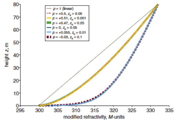
Fig. 2 Modelling three sub-refractive profiles, using various values of z_0 . Refractivity profiles for M(0) = 300 , M(80) = 332 and G_M = 0.12 M -units/m, for the usual linear assumption p = 1 , and two nonlinear profiles, each generated firstly with z_0 = 0.05 m, and then super-imposed profiles with smaller and larger z_0 values, produced by adjusting the value of p in (4)
