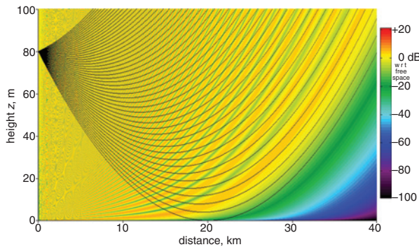
Fig. 3 Predicted field relative to free-space, and ray tracing, for p=1 Sub-refraction +400 M-units/km: M(0)=300 , M(80)=332 Transmitter: 10 GHz at 80 m, with traced rays 0.2 milliradians apart
