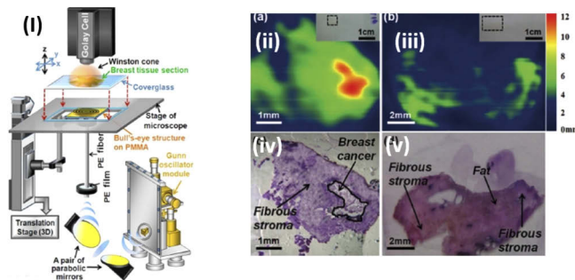
Fig. 13. Schematic of the all-terahertz fiber scanning near-field microscope. Here, (ii) and (iii) are terahertz near-field absorption coefficient images of the breast tissue sections, cancerous and normal samples, respectively. Also, (iv) and (v) are photomicrographs of the corresponding breast tissue.
