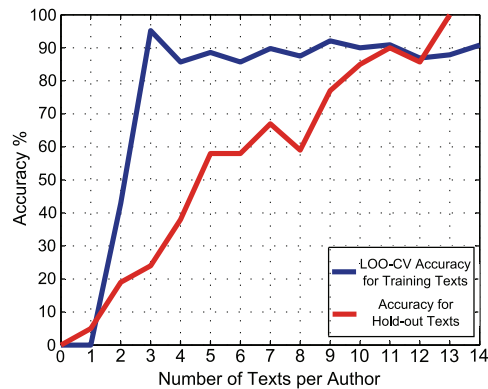
Figure 2. Number of texts per author vs. accuracy of MDA classifier. This graph investigates accuracy versus the size of the training dataset for the MDA case, with a fixed set of 100 function words, for the benchmark English corpus of known texts given in Table 1. The upper curve shows the LOO-CV accuracy of MDA, as a function of the number of author texts, by deliberately limiting the size of the training dataset. The lower curve shows the MDA accuracy that is obtained by inputting the hold-out texts to the classifier at each step. doi:10.1371/journal.pone.0054998.g002
