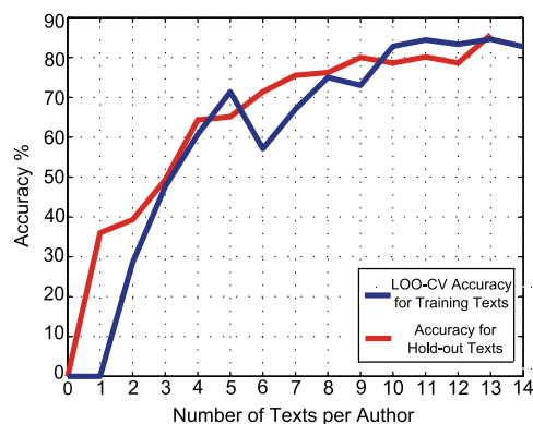
Figure 3. Number of texts per author vs. accuracy of SVM classifier. This graph investigates accuracy versus the size of the training dataset for the SVM case, with a fixed set of 95 function words, for the benchmark English corpus of known texts given in Table 1. The SVM utilizes a polynomial kernel with \gamma = 2^{-12} , r = 2^{11} and d = 3 . doi:10.1371/journal.pone.0054998.g003
