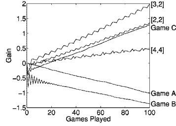
FIGURE 1. The progress of playing games A and B. Simulations were performed by playing game A a times, game B b times, and so on until a total of 100 games were played. This is represented by [a, b] . The results were averaged from 50 000 trials using Parrondo's original numbers with \varepsilon = 0.005 .
