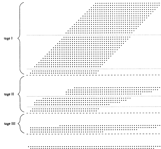
Figure 6. One possible reduction scheme for 32 \times 32 partial product matrix
