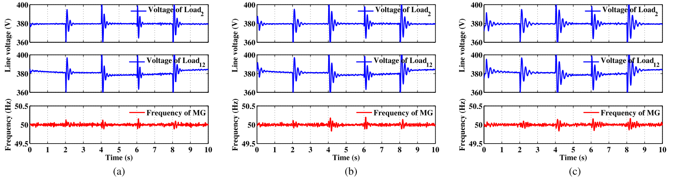
Fig. 6. Simulation results under different time delays, when both environmental conditions and load demand fluctuate over time. (a) \alpha = 10 ms, (b) \alpha = 20 ms, (c) \alpha = 30 ms.
