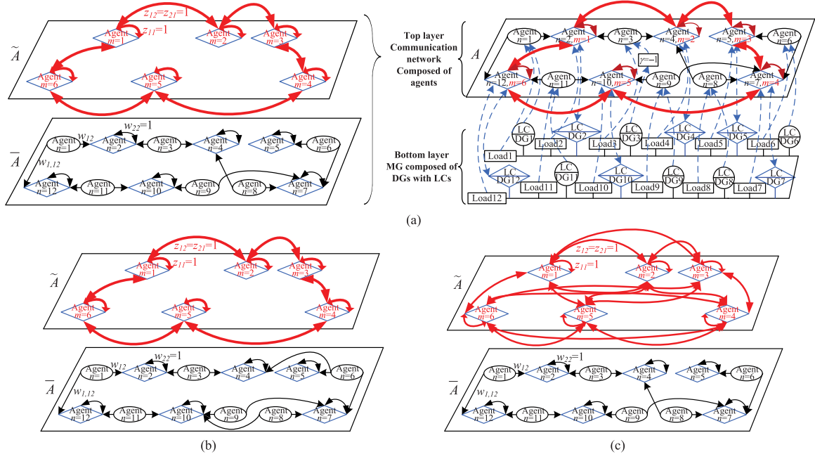
Fig. 1. Two-layer control model for an MG, where uncontrollable and partially controllable agents are indicated by circles, while controllable agents are indicated by diamonds. (a) Network 1. The left panel is the subgraph \bar{A} composed of n agents and the subgraph \bar{A} composed of m controllable agents. The right panel is the communication network A = G(V, E) and the MG. (b) Network 2. (c) Network 3.
