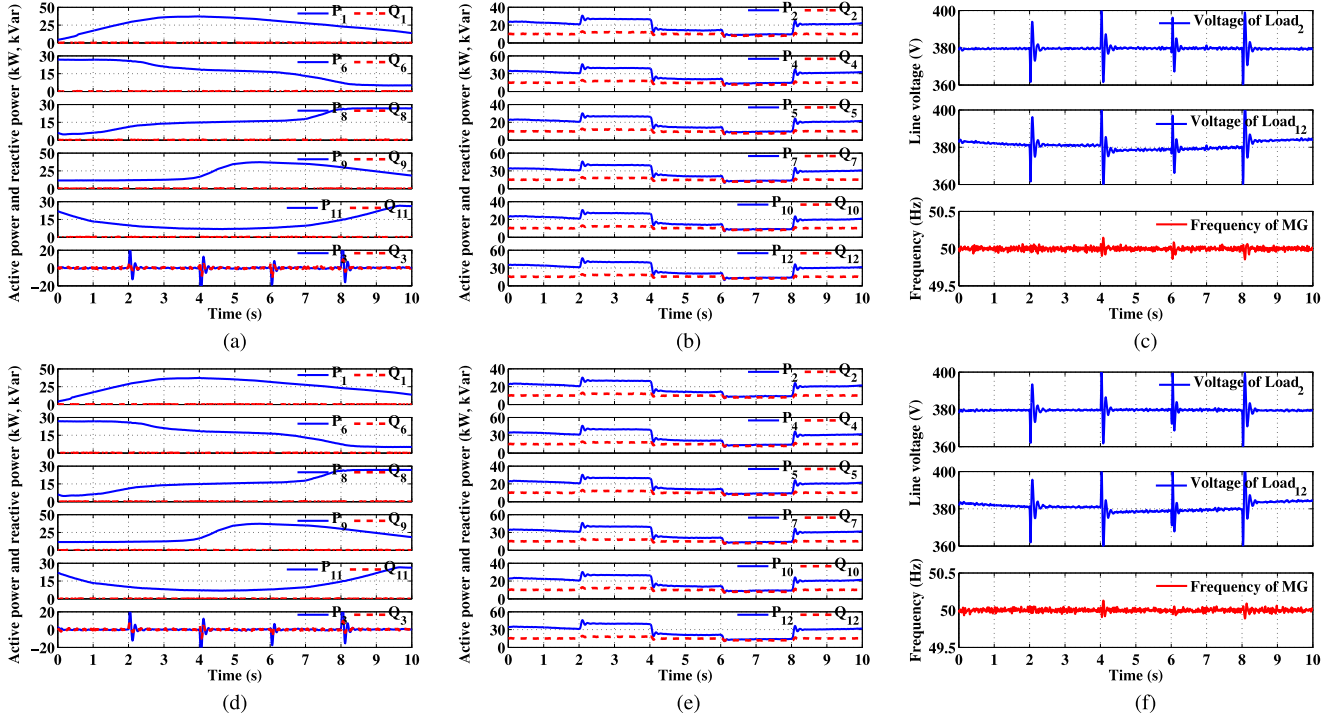
Fig. 5. Simulation results under different topologies, when both environmental conditions and load demand fluctuate over time. (a), (d) Active and reactive power outputs of uncontrollable and partially controllable. (b), (e) Active and reactive power outputs of controllable DGs. (c), (f) The line voltages and frequency in the MG. (a)–(c) On Network 2. (d)–(f) On Network 3.
