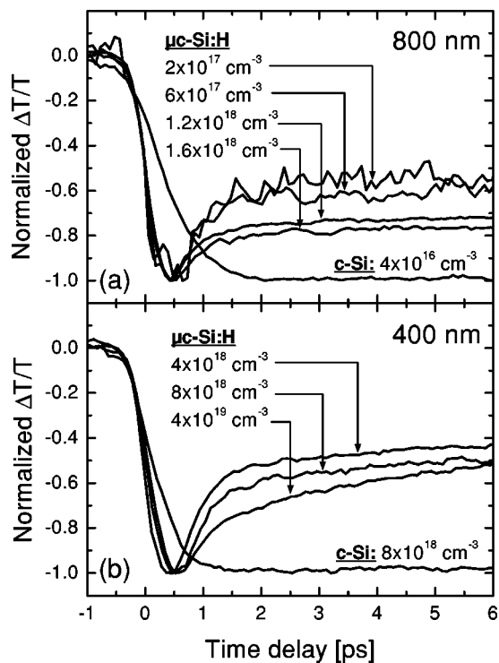
FIG. 1. Normalized THz transmission transients obtained subsequent to (a) 800 nm and (b) 400 nm excitation. Transients recorded on c -Si are shown for comparison. Excitation densities are indicated with arrows in the figure.
