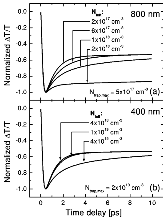
FIG. 2. (a) Numerically calculated transients using parameters as in Fig. 1(a) for 800 nm excitation, and (b) parameters as in Fig. 1(b) for 400 nm excitation.
