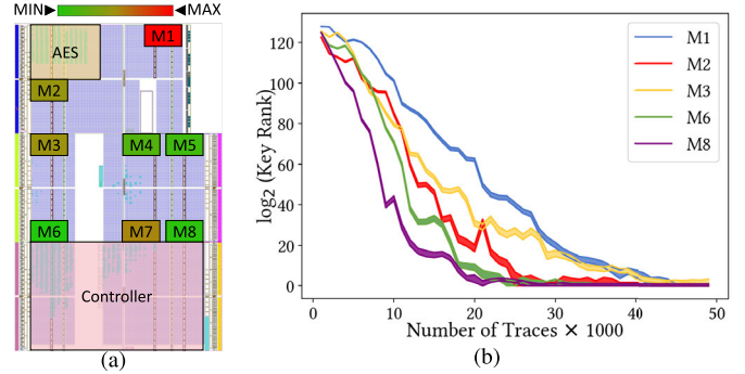
Fig. 10. KR estimation for MUXLeak. The curves in (b) are named after the number on each placement shown in (a).
