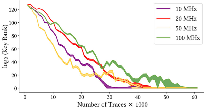
Fig. 11. Impact of the AES frequency on our attack. MUXLeak has the capability to expose the entire AES key within 60k traces across various operating frequencies under the worst placement, i.e., M1 in Fig. 10(a).
