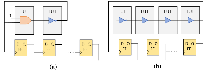
Fig. 3. Examples of the RO circuit design. All of them contain a combinational loop where the signal propagates through a series of logic gates and is ultimately fed back to itself. (a) RO circuits in [58]. (b) RO circuits in [14].
