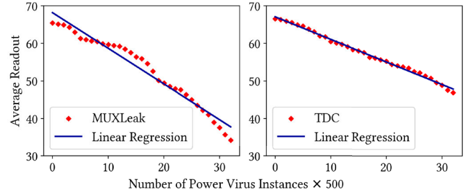
Fig. 8. Sensitivity of MUXLeak and TDC [18] in the same placement under different victim activities.
