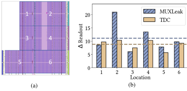
Fig. 9. Sensitivity of MUXLeak and TDC [18] under different placements. The index as the x -axis in (b) corresponds to the region index in (a). The dashed line indicates the average value of a sensor.
