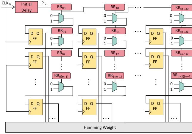
Fig. 4. Overview of MUXLeak.
