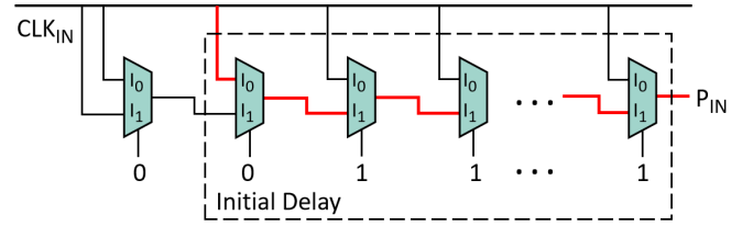
Fig. 7. MUX-based calibration design. The red line denotes the actual signal propagation path. When the last c select signals are configured as "1," CLK_{IN} is required to go through c+1 MUXes (within the dashed box) before reaching P_{IN} .
