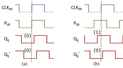
Fig. 6. Example timing diagram of (a) uncalibrated and (b) calibrated MUXLeak. The vertical dotted line shows a rising edge of the CLK_{IN} . Q_{ij} denotes the output of FF_{ij} in an idle PDN, while Q_{ij}' denotes the same output in a busy PDN.
