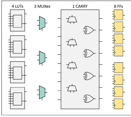
Fig. 1. Each slice in the Xilinx 7 series architecture encompasses four types of basic resources: four LUTs, one CARRY, eight FFs, and three MUXes. Two slices are combined to form a CLB.
