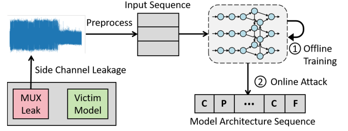
Fig. 12. MUXLeak-based model architecture stealing.
