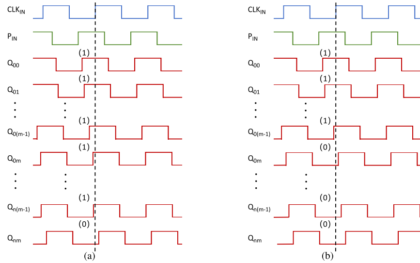
Fig. 5. Example timing diagram of MUXLeak. The impact of PDN instability is exaggerated to amplify the visual clarity. (a) Idle PDN. (b) Busy PDN.
