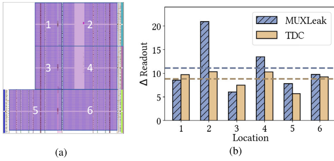
Fig. 9. Sensitivity of MUXLeak and TDC [18] under different placements. The index as the x-axis in (b) corresponds to the region index in (a). The dashed line indicates the average value of a sensor.
